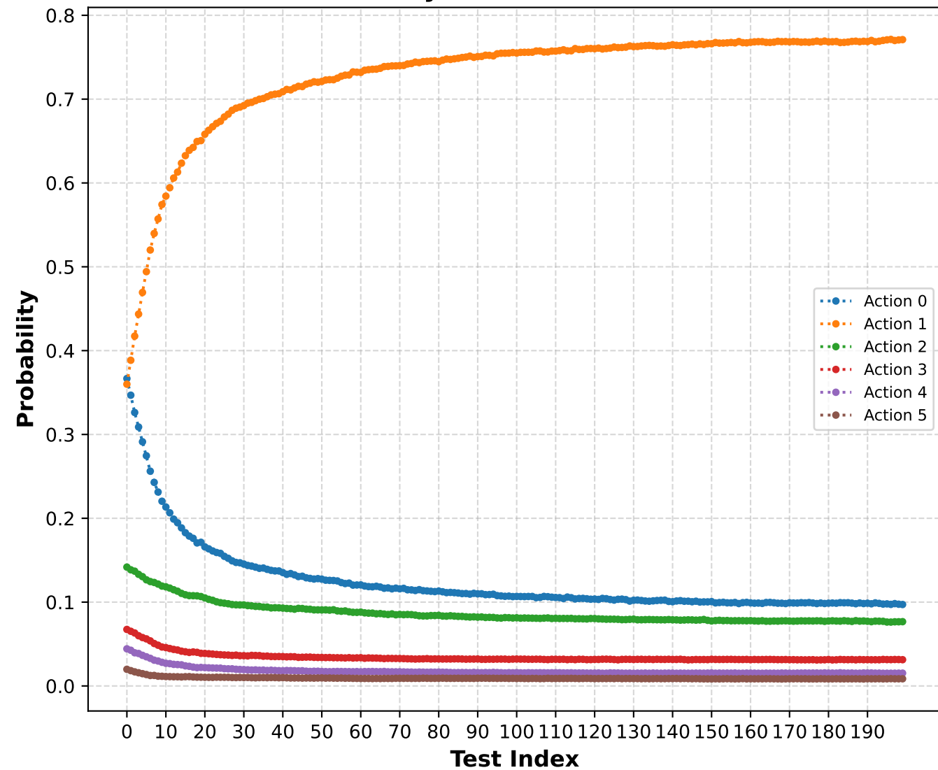
Action Probability Evolution M = 100, N = 160
